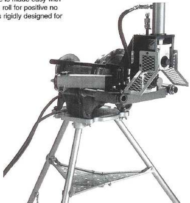
Model 1012 Roll Groover for Mounting on Ridgid® 300 Pipe Threader.
